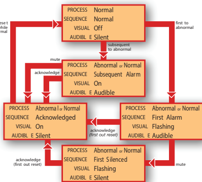
MANUAL RESET FIRST OUT WITH NO SUBSEQUENT ALARM FLASHING AND SILENCE PUSHBUTTON N Sequence F2M-1
